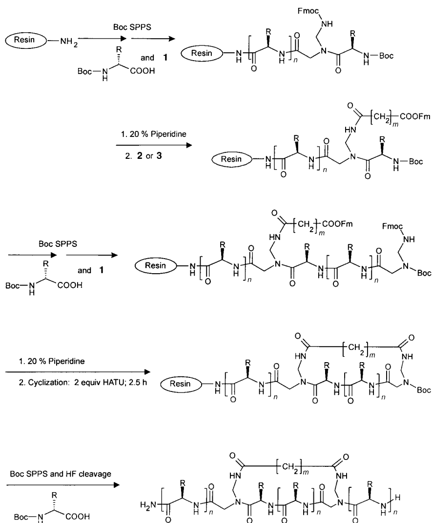
Scheme 3. General strategy for the synthesis of N-backbone cyclic peptide analogues of the AA 42-61 N-terminal MSP-1 fragment. HATU = N [(dimethylamino)-1 H -1,2,3-triazole[4,5- b ]-pyridin-1-ylmethyl]- N -methylmethanaminium hexafluorophosphate.
