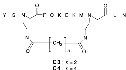
Scheme 1. Linear and cyclic peptide analogues of the AA 42–61 N-terminal MSP-1 fragment.
